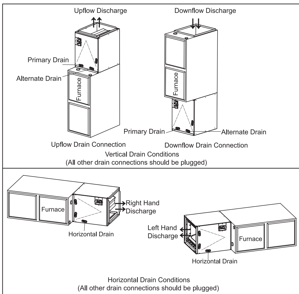
Fig. 3-1 INSTALLATION OF CASSED COIL
